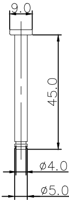
MS-5-45-E
