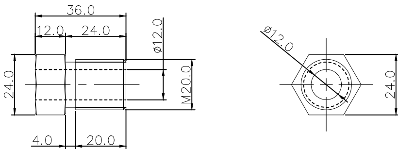
L-3T4 (BOLT)
