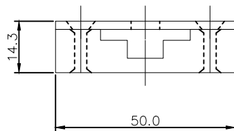
INTER-LOCK ASS'Y
