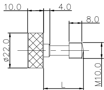
BOLT LOCKER
