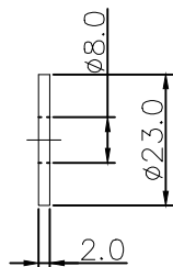
RUBBER WASHER
