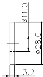
FLAT WASHER
